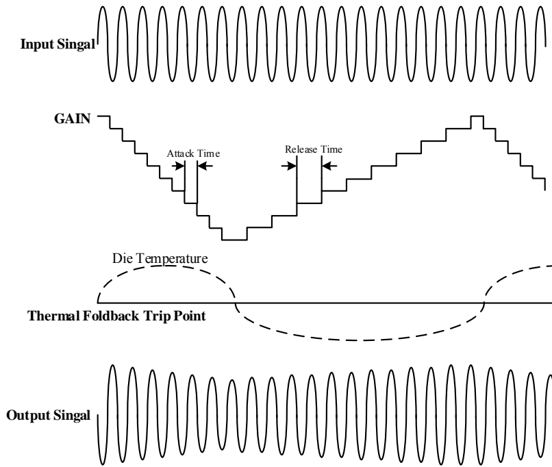
Fig. 3 Thermal Foldback Operation
